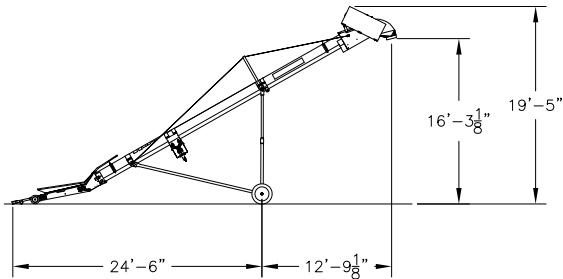
ELECTRIC DRIVE AT MAXIMUM INCLINE
