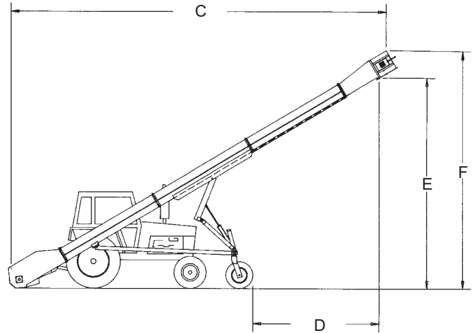
Side View in Loading Position
