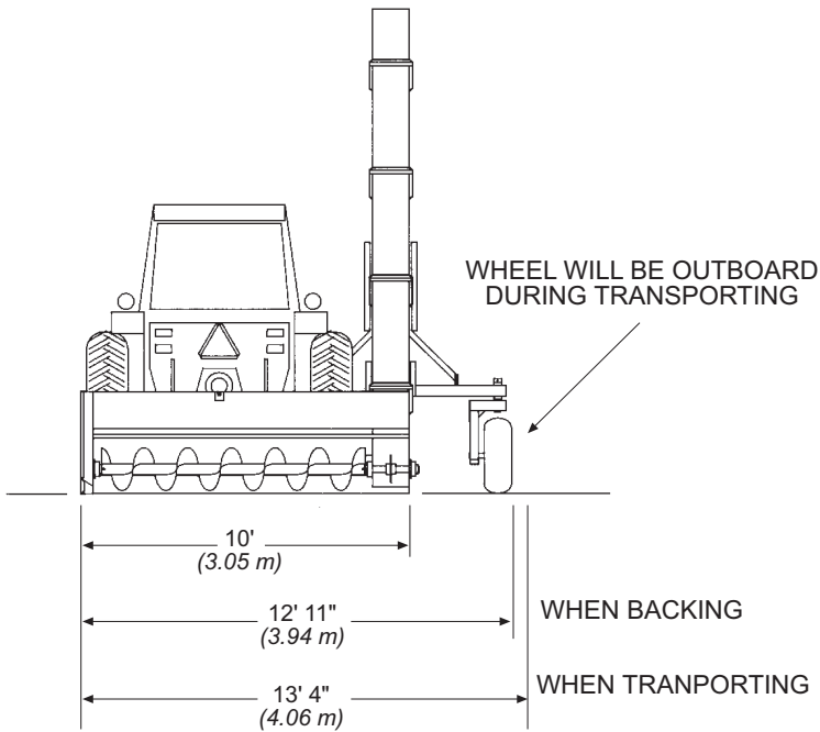
Back View
