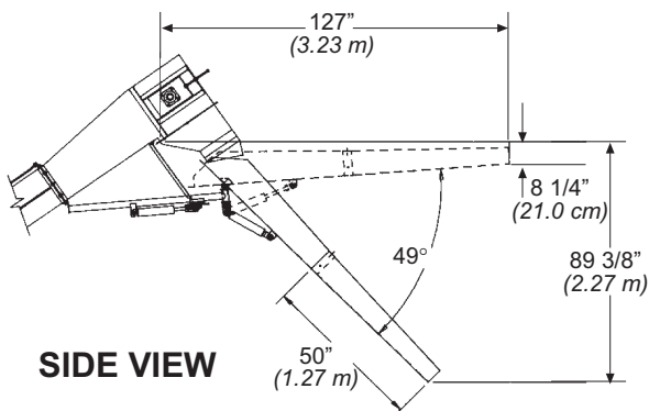
Optional Hydraulic Swivel Spout (MT9013)
