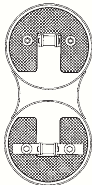
CROSS SECTION OF HOUSING
