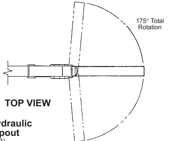
Optional Hydraulic Adjustable Spout (MT9011)
