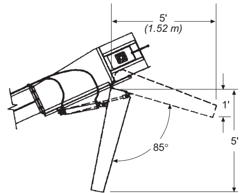
Optional Hydraulic Adjustable Spout (MT9011)
